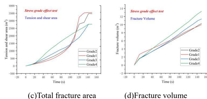
Fig. 2 Stress grade - fracture characteristic parameters
